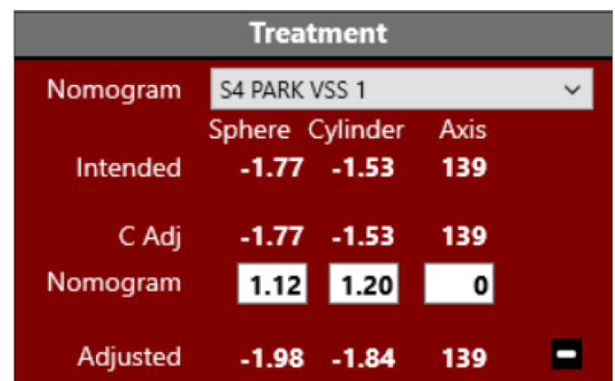
Figure 6: Vector planning
